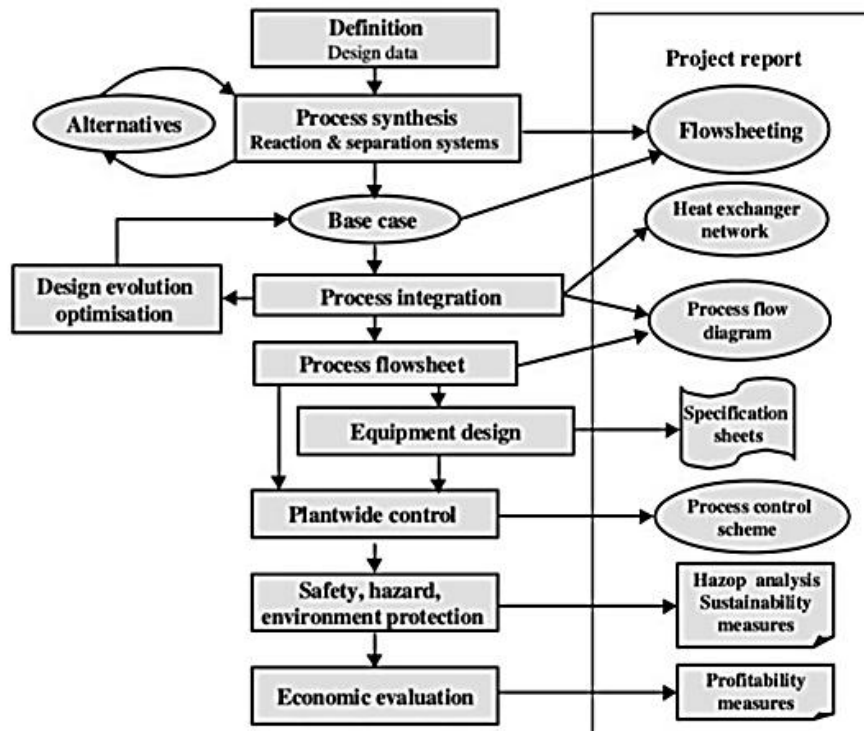
Figure 1.1 Outline of a design project.
